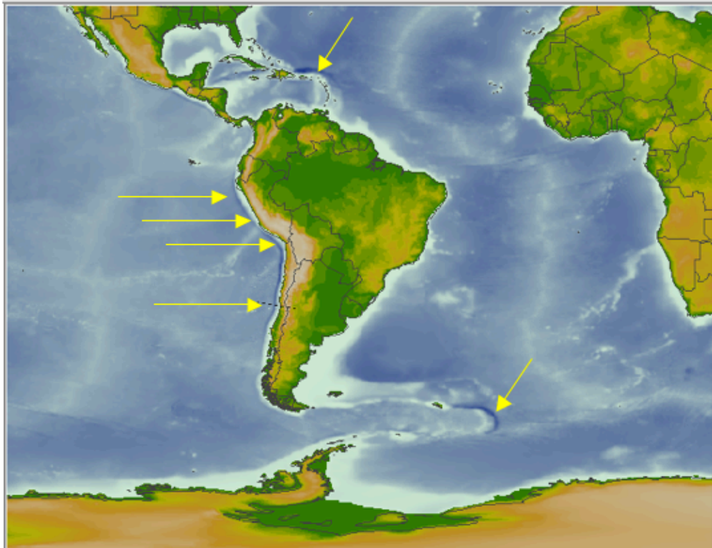
Global Elevation and Bathymetry Elevation (m) -9,000 0 9,000
